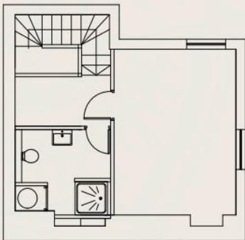
Fifth Floor
