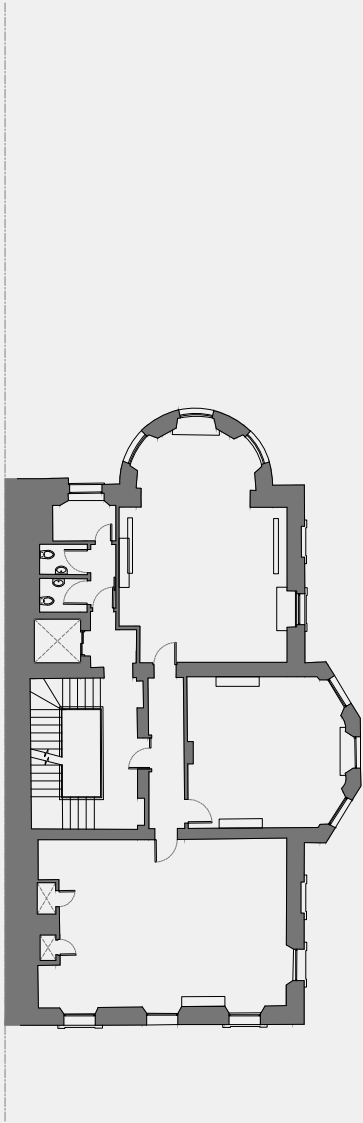
Fig.15 Existing second floor plan
